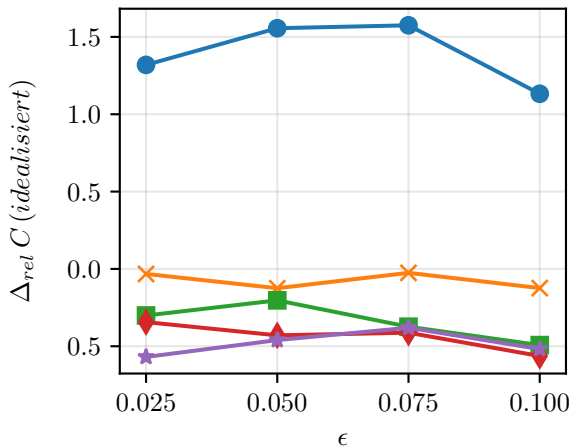
Barrier Option - Festgitter - Cutoff
