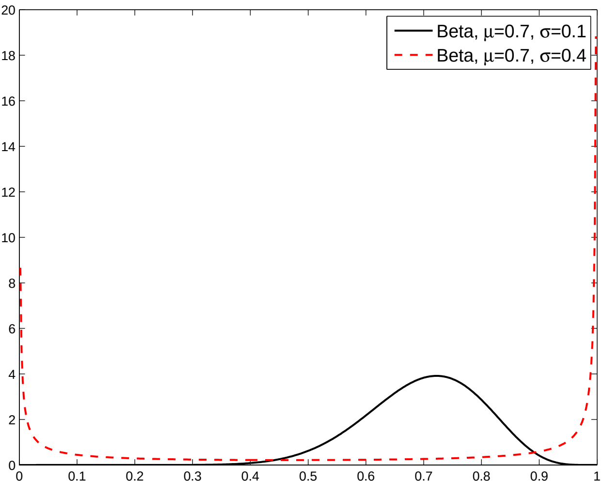
Beta Prior
