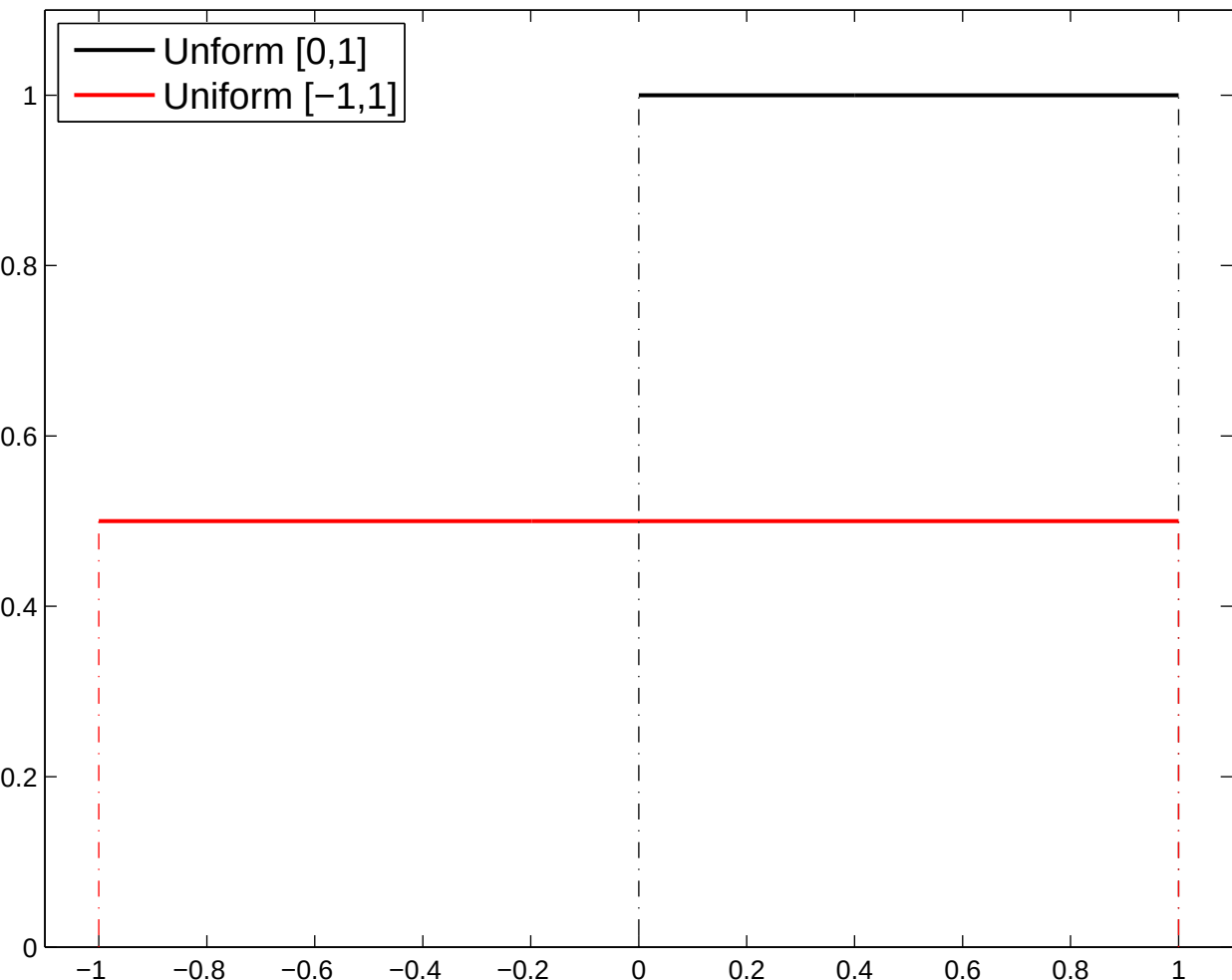
Uniform Prior
