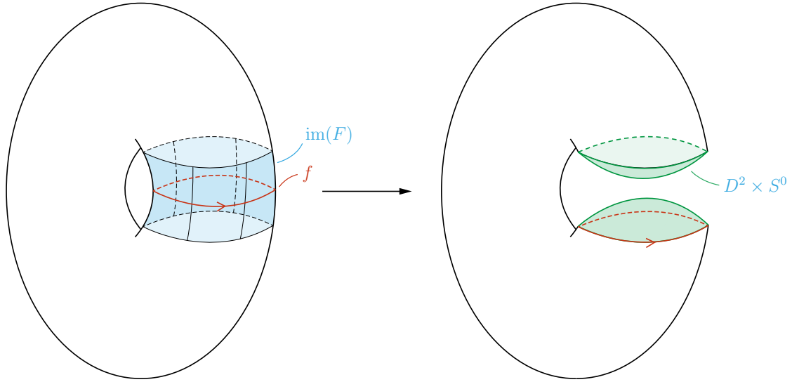
Figure 1: Performing a 1-surgery on the Torus to kill the homotopy class represented by f . The resulting space is a 2-sphere, where the corresponding class is now trivial.
