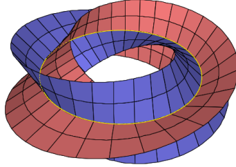
Figure 2: Illustration of the Whitney sum of two Moebius bundles [source: https://math.stackexchange.com/questions/1009126/global-trivialization-of-f-m-oplus-m ]
