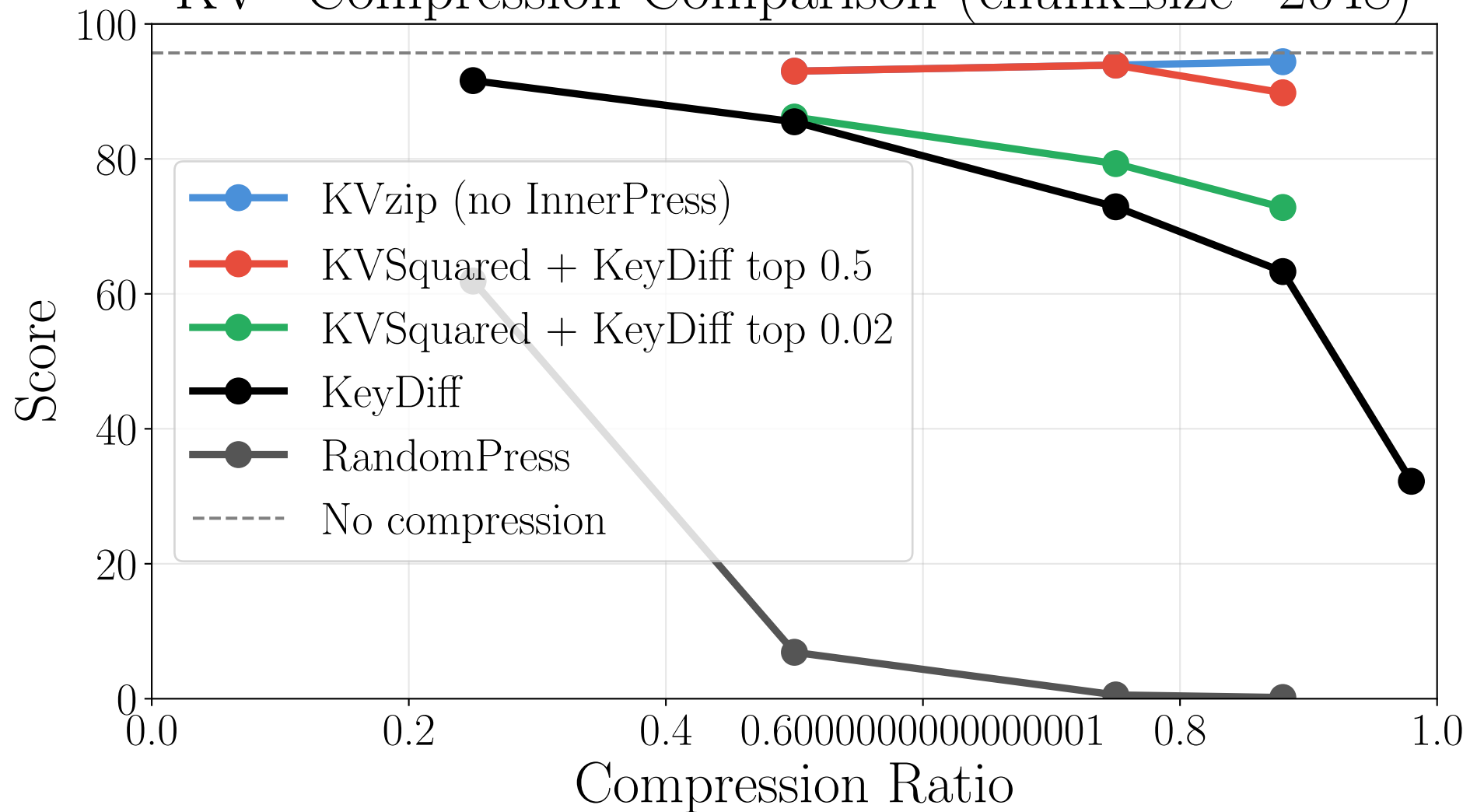
KV 2 Compression Comparison (chunk_size=2048)
