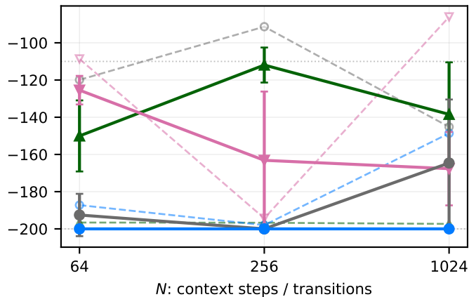
MountainCar
