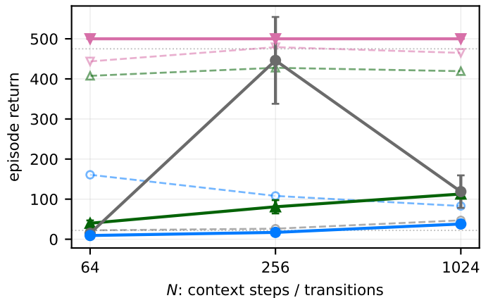
CartPole
