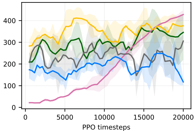
CartPole: return inside the model
