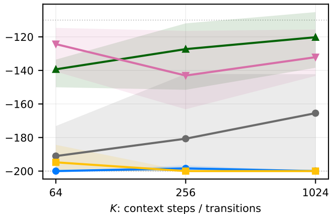
MountainCar
