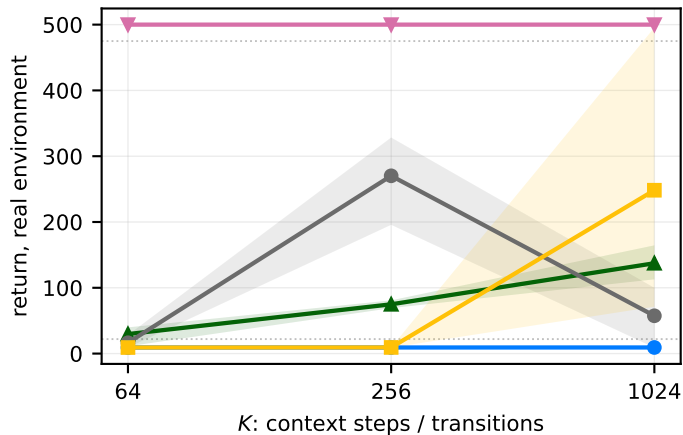
CartPole
