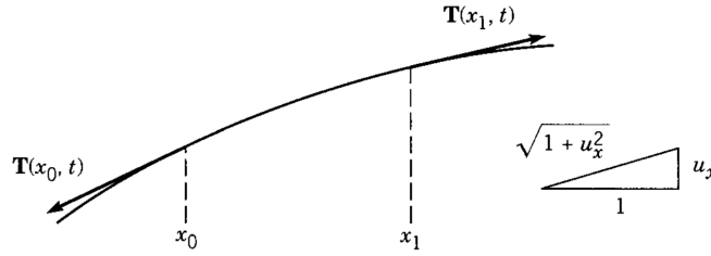
Figure 3: A zoomed vibrating string ( Source: Strauss PDE )
