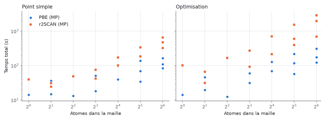
Figure 2: Total time versus number of atoms on one GPU.
