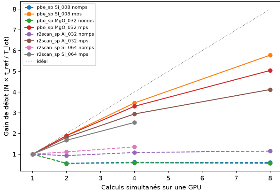
Figure 5: Throughput gain of N concurrent single points on one GPU. Solid lines: with MPS; dashed lines: without MPS; dotted line: ideal gain.
