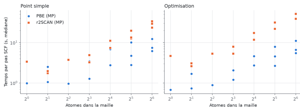
Figure 1: Median time per SCF step versus number of atoms on one GPU.
