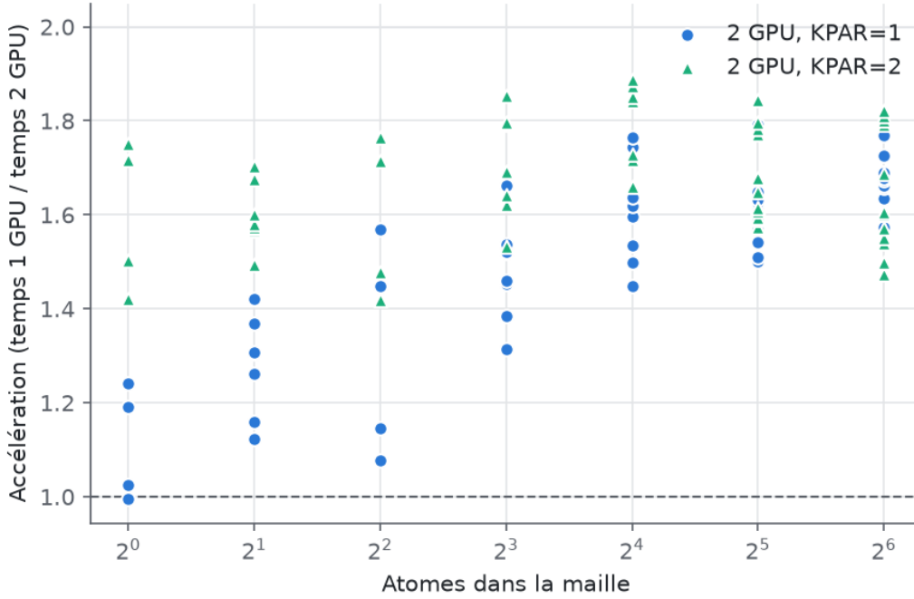
Figure 3: Speedup on two GPUs versus number of atoms, for KPAR=1 (g2k1) and KPAR=2 (g2k2).
