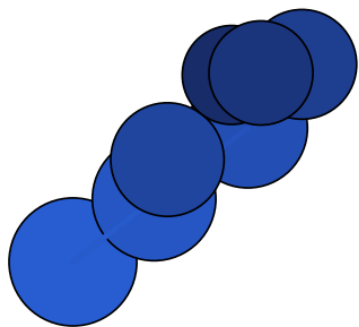
N7_anion_anion_001 – C1 – \Delta H = 0.00 (DFT) – our work
