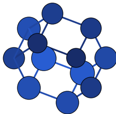
N12_neutral_neutral_009 – D6h – \Delta H = 334.92 (DFT) – our work
