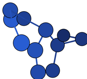
N11_anion_anion_013 – C1 – \Delta H = 116.68 (DFT) – our work
