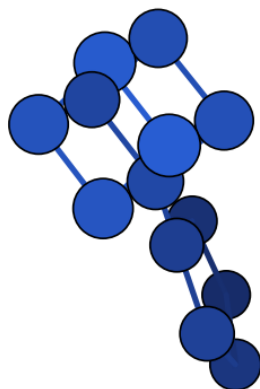
N13_cation_cation_004 – C1 – \Delta H = 151.22 (DFT) – our work
