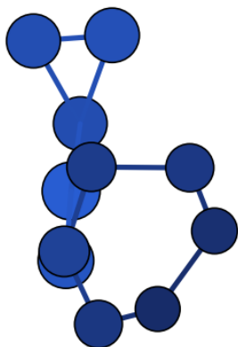
N11_cation_cation_006 – C1 – \Delta H = 44.38 (DFT) – our work
