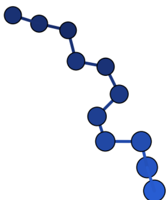
N11_anion_anion_006 – C1 – \Delta H = 0.00 (DFT) – our work
