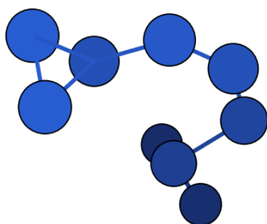
N9_anion_anion_018 – C1 – \Delta H = 98.82 (DFT) – our work
