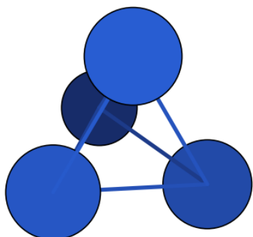
N4_neutral_neutral_001 – Td – \Delta H = 0.00 (DFT) – our work
