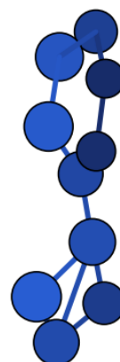
N10_neutral_neutral_014 – C1 – \Delta H = 139.29 (DFT) – our work
