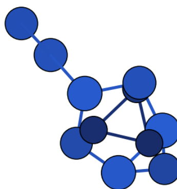
N11_cation_cation_007 – C1 – \Delta H = 118.69 (DFT) – our work
