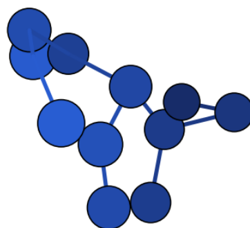
N11_anion_anion_013 – C1 – \Delta H = 177.01 (DFT) – our work
