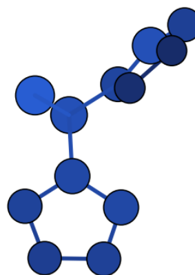
N12_neutral_neutral_003 – C1 – \Delta H = 36.41 (DFT) – our work
