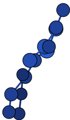
initiale (xTB, N 14 0 intact)
