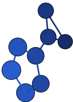
N8_neutral_neutral_013 – C2 – \Delta H = 101.43 (DFT) – our work
