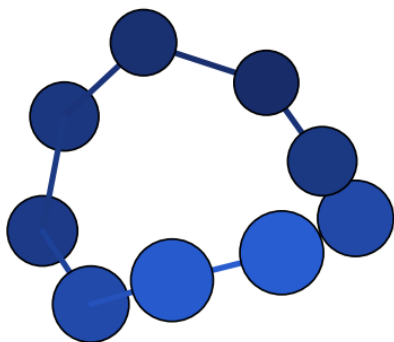
initiale (xTB, N_9^+ )
