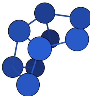
N9_anion_anion_013 – C1 – \Delta H = 96.48 (DFT) – our work
