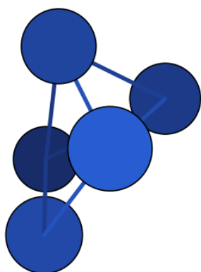
initiale (xTB, intacte, N_5^+ )
