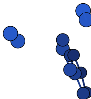
dernier cycle DFT (50 cycles)
