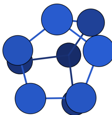
N9_cation_cation_011 – Cs – \Delta H = 82.84 (DFT) – our work
