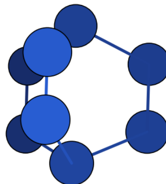
N8_neutral_neutral_009 – D3h – \Delta H = 68.56 (DFT) – our work
