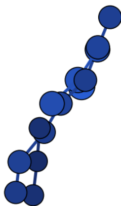
initiale (xTB, N 14 0 intact)
