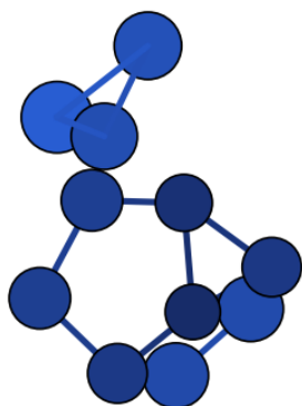
initiale (xTB, N_{11}^{1-} intact)
