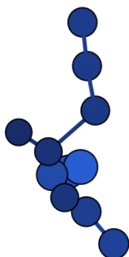
initiale (xTB, N_{11}^{1-} intact)
