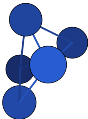
initiale (xTB, N_5^+ intact)
