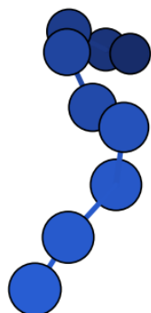
initiale (xTB, N_9^+ intact)
