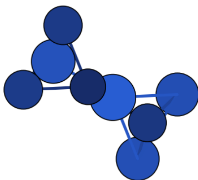
N8_neutral_neutral_023 – D2h – \Delta H = 183.12 (DFT) – our work
