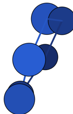
N6_neutral_neutral_002 – D2 – \Delta H = 195.83 (DFT) – our work – N–N > 1,7 Å
