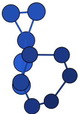
N11_cation_cation_006 – C1 – \Delta H = 67.68 (DFT) – our work – N–N > 1,7 Å
