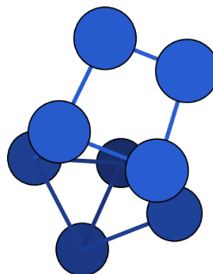
N8_neutral_neutral_016 – Cs – \Delta H = 122.30 (DFT) – our work
