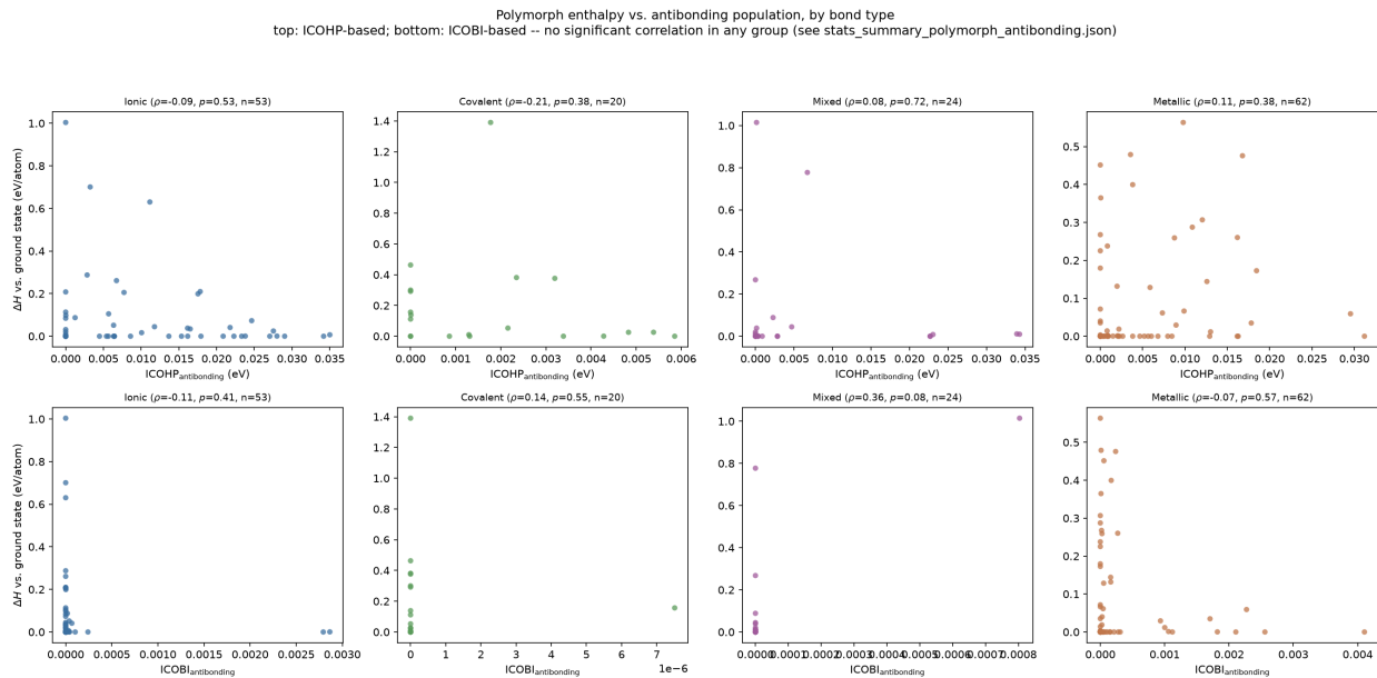
Figure 4: Polymorph enthalpy above the same-formula ground state versus raw antibonding population, one column per icobi_label bond-type group, ICOHP-based (top row) and ICOBI-based (bottom row).
