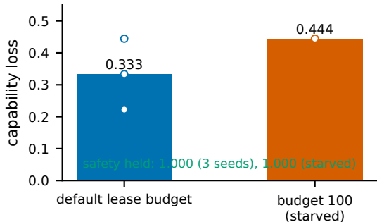
Fig. 3 Death is capability loss, never a safety bypass
