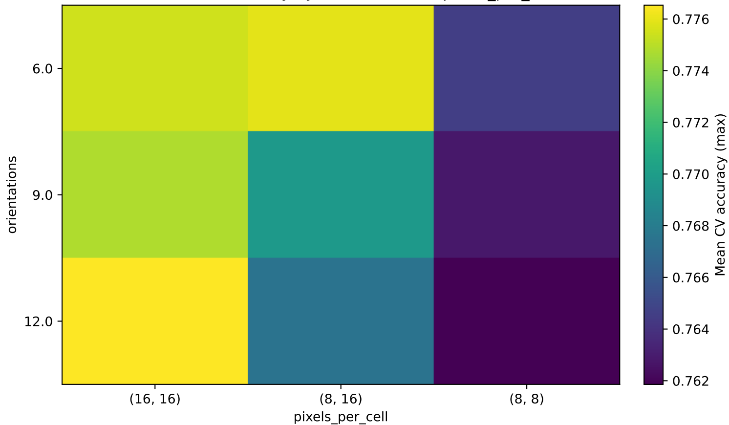
HOG — max accuracy by (orientations × pixels_per_cell)
