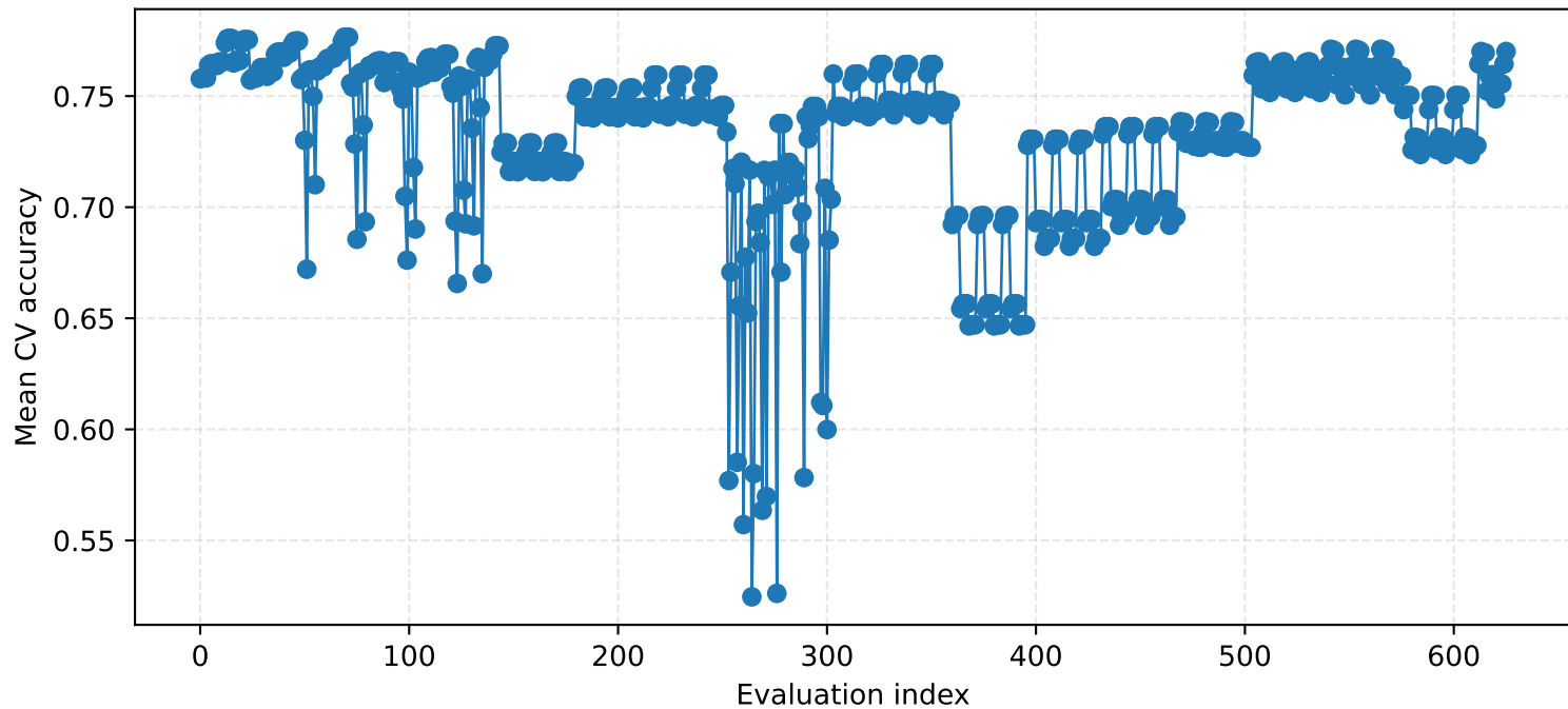
Grid search progress
