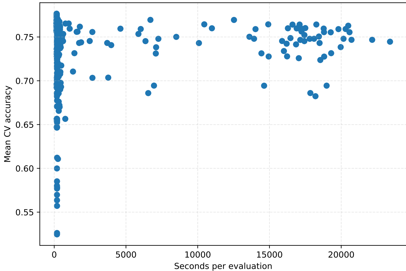
Runtime vs accuracy
