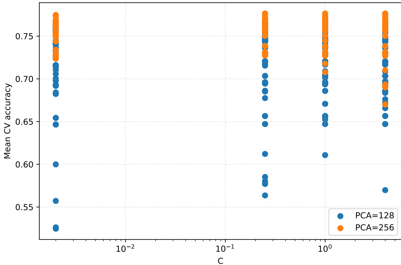
Accuracy vs C
