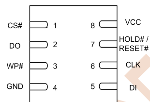
Figure 3.2 8-Contact 6 x 5 mm WSON
