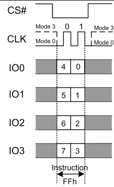
Figure 7.42 Exit QPI Instruction (QPI Mode only)
