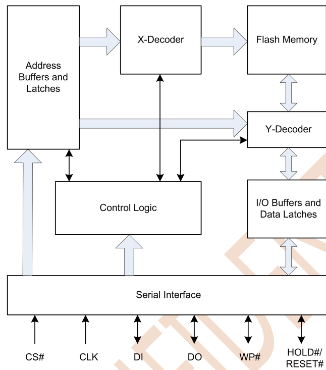
Figure 2.1 Block Diagram
