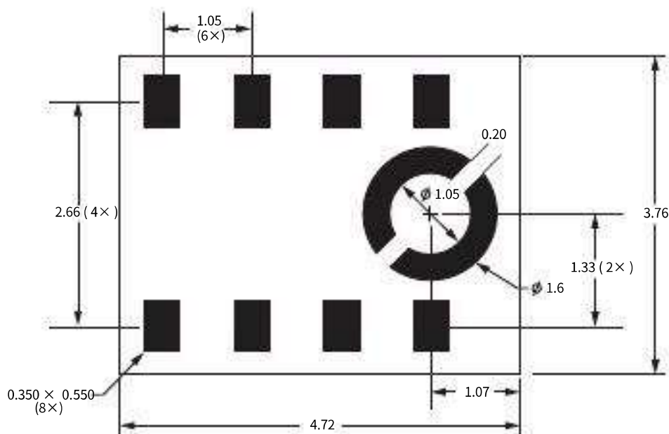
Figure 14. Suggested PCB Land Pattern Layout
