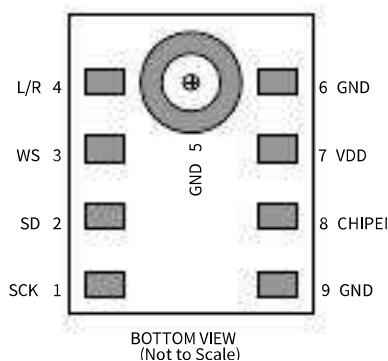
Figure 3. Pin Configuration
