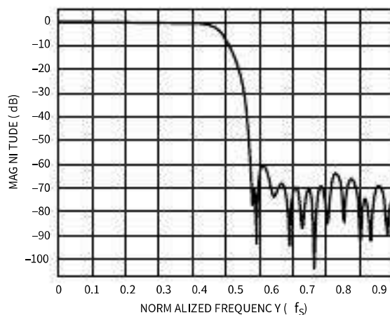
Figure 12. Digital Low-Pass Filter Magnitude Response
