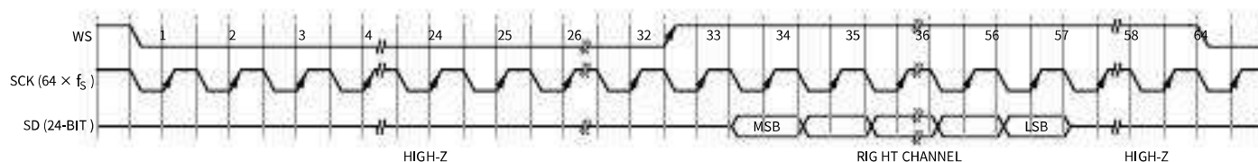
Figure 10. Mono-Output I²S Format Right Channel (L/R = 1)
