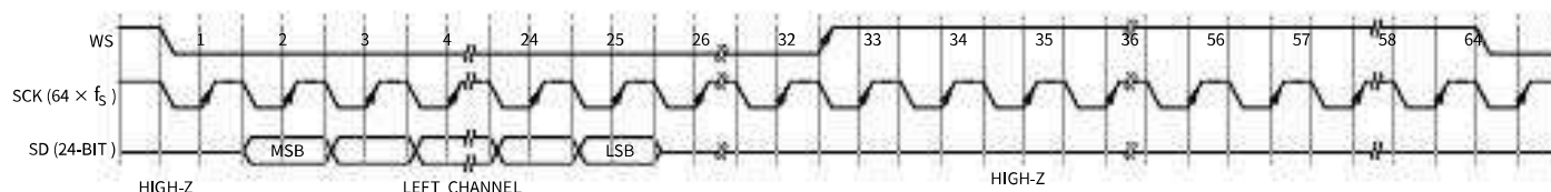
Figure 9. Mono-Output I²S Format Left Channel (L/R = 0)
