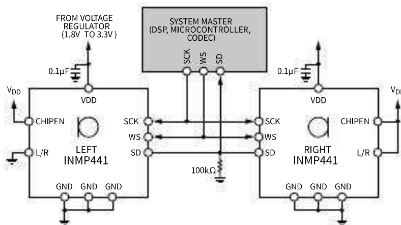
Figure 7. System Block Diagram
