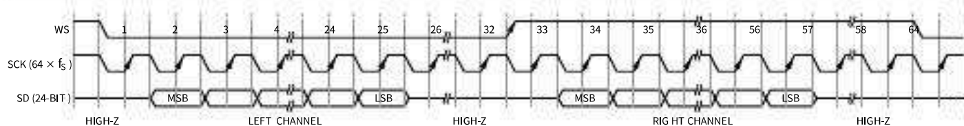
Figure 8. Stereo-Output I²S Format
