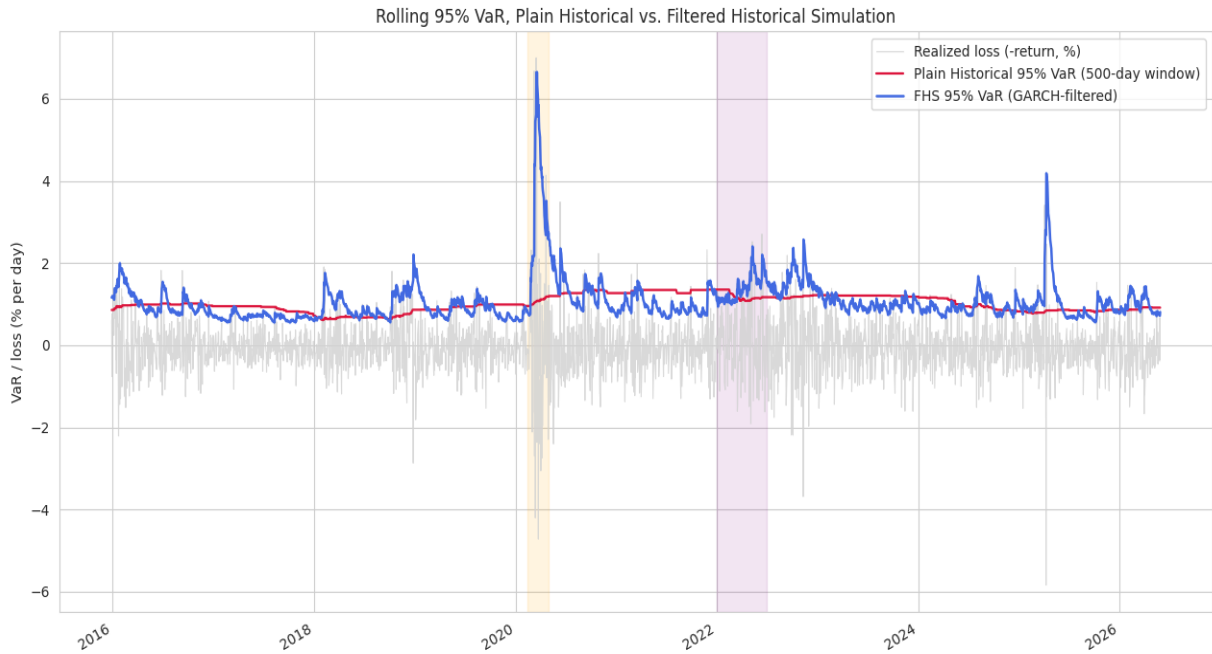
Figure 3, The headline chart of the project. Plain Historical VaR (red) lags by months because it averages over a 500-day window; FHS (blue) reacts the next day, because \sigma_t spikes immediately when markets move.
