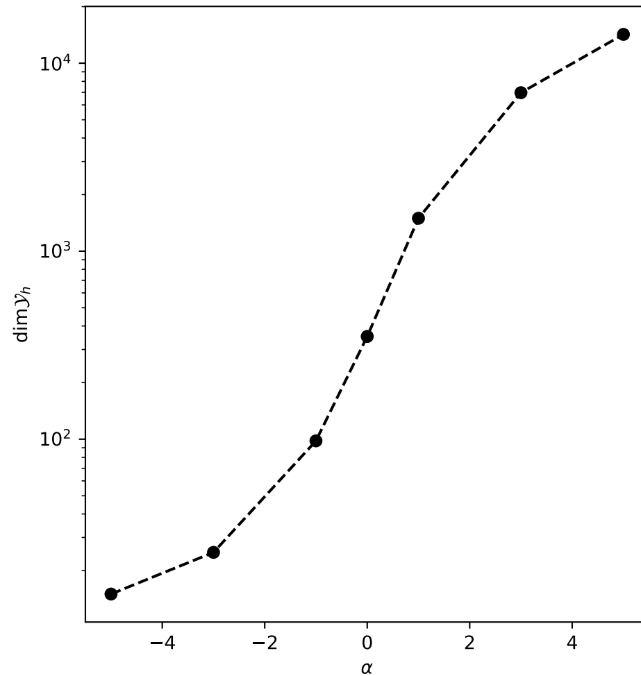
Dimension of \mathcal{Y}_h required to obtain 99.9% of H^\alpha Energy
