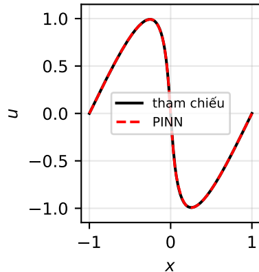
(b1) t = 0.25
