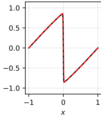
(b3) t = 0.75
