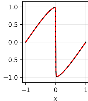
(b2) t = 0.50
