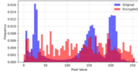
Camerman - Histogram Comparison
