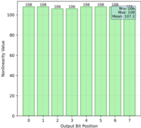
Component Nonlinearities
