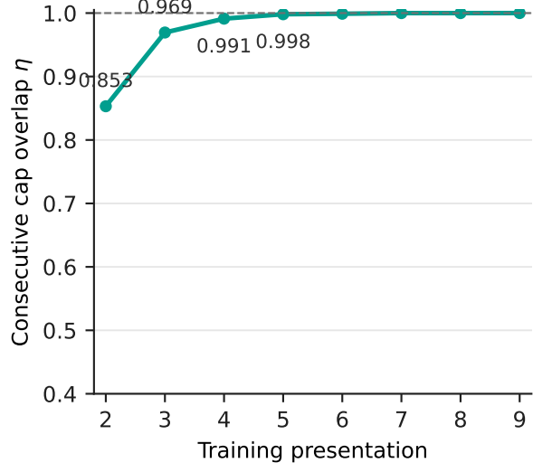
Formation transient
