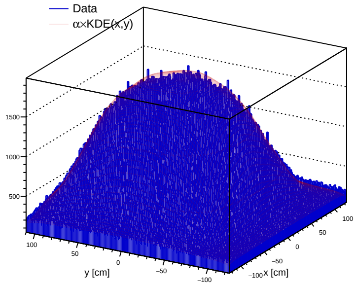
Weighted, adaptive, mirrored/unmirrored KDE
