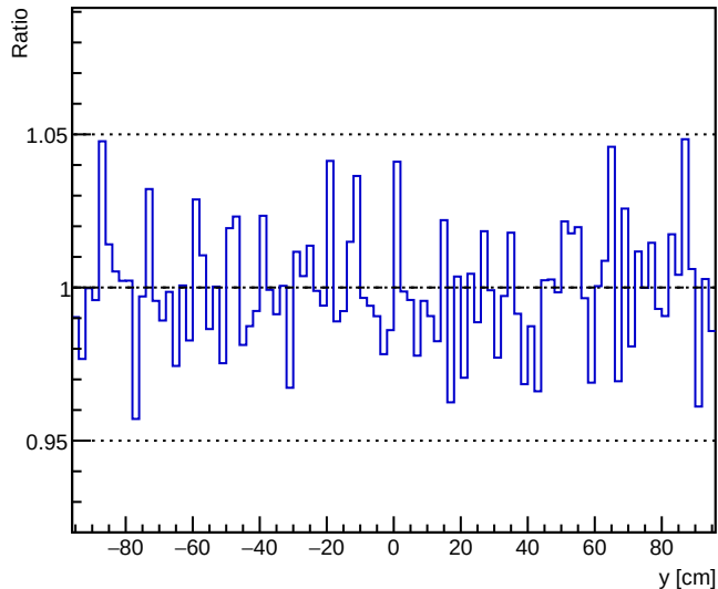
-100um x shift / nominal MM1 Y Projection
