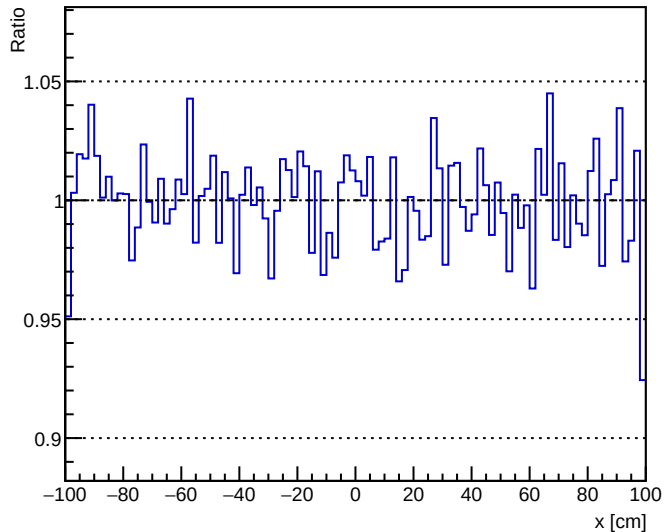
-100um x shift / nominal MM1 X Projection
