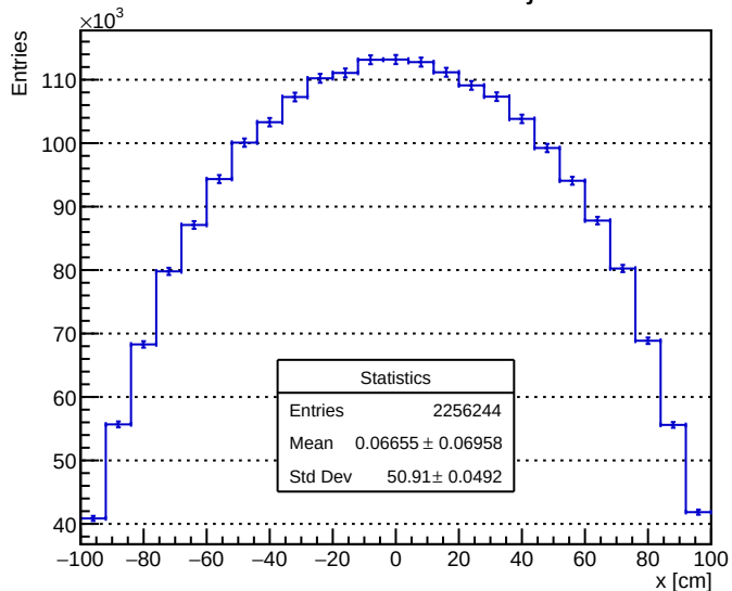
+100um x shift MM1 X Projection
