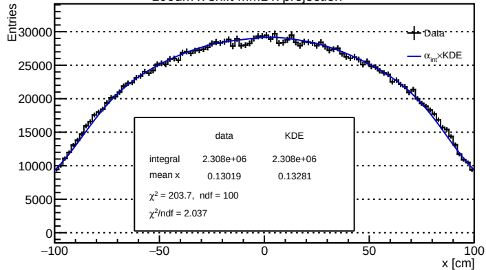
-100um x shift MM1 x projection
