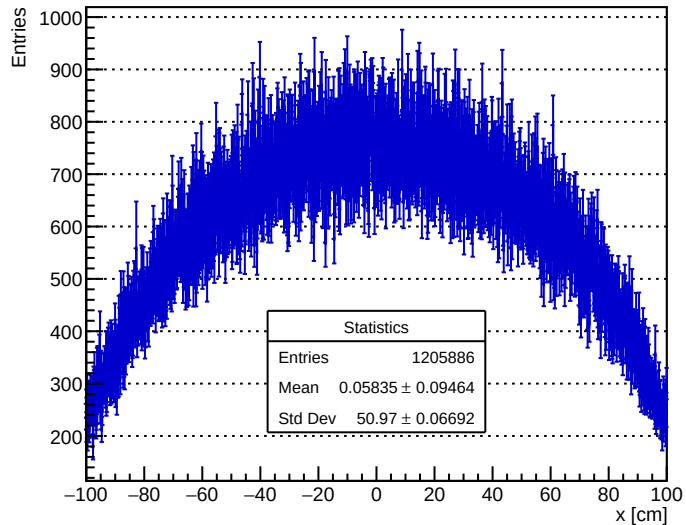
+X 100um Beamshift X Projection
