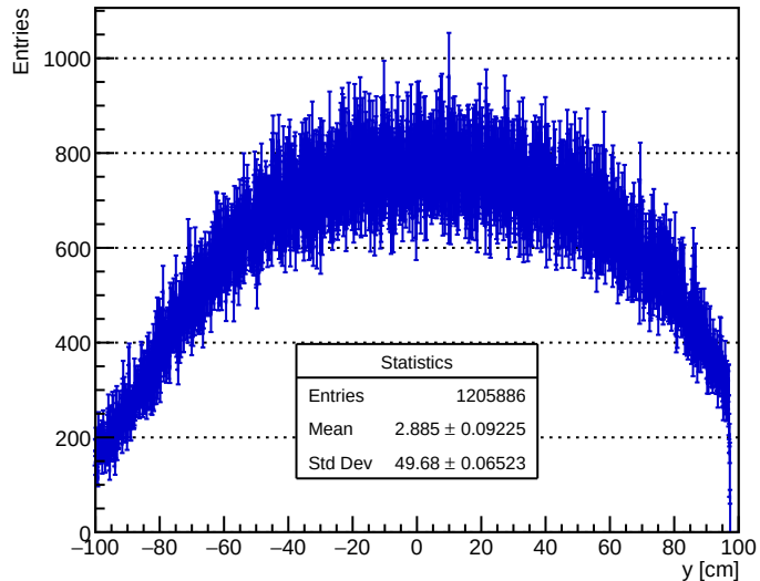
+X 100um Beamshift Y Projection
