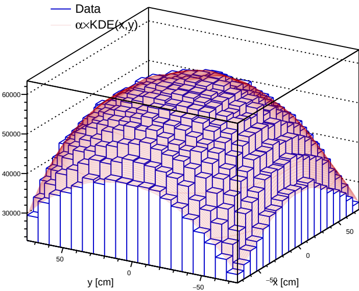
Weighted, adaptive, mirrored/unmirrored KDE
