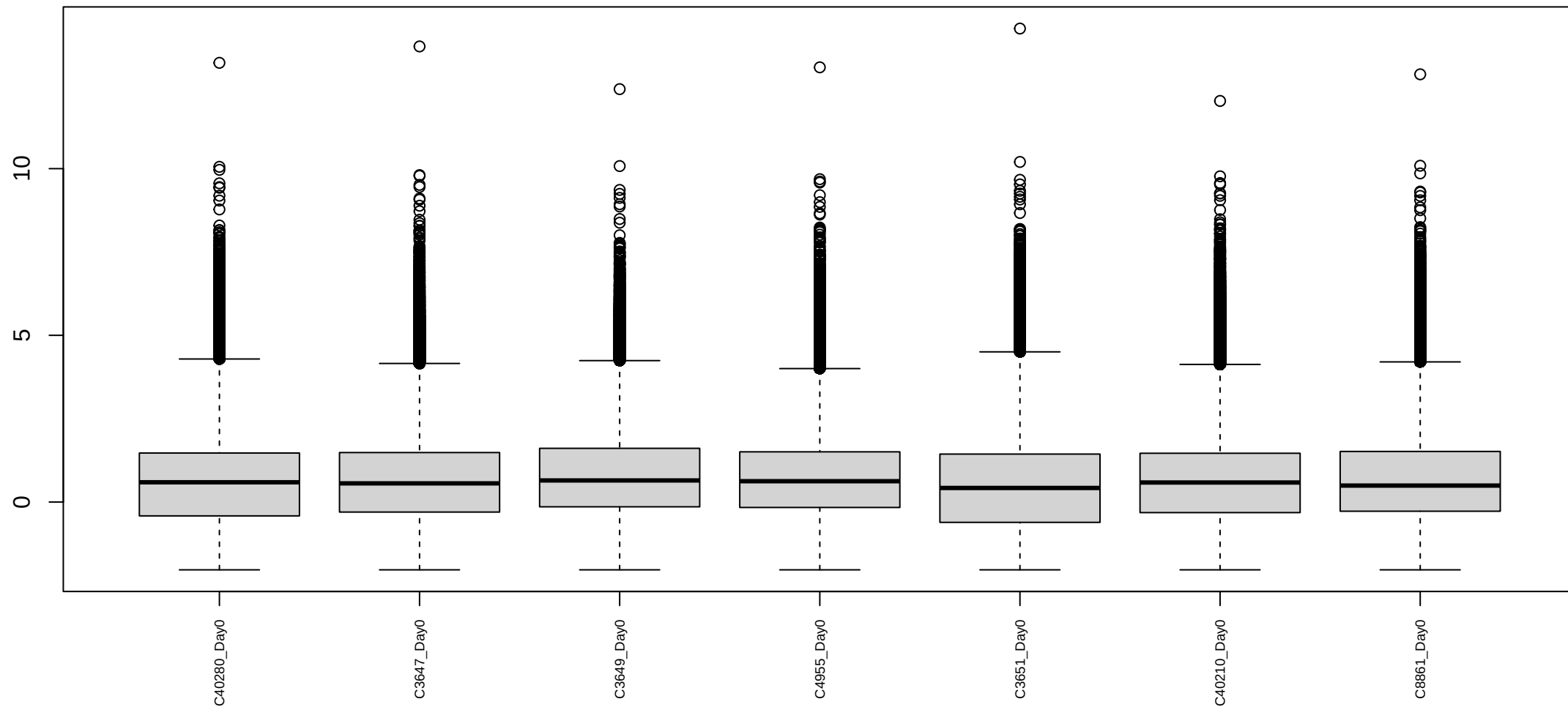
Boxplots of log cpm per sample Chimp Day 0 Reproducible2
