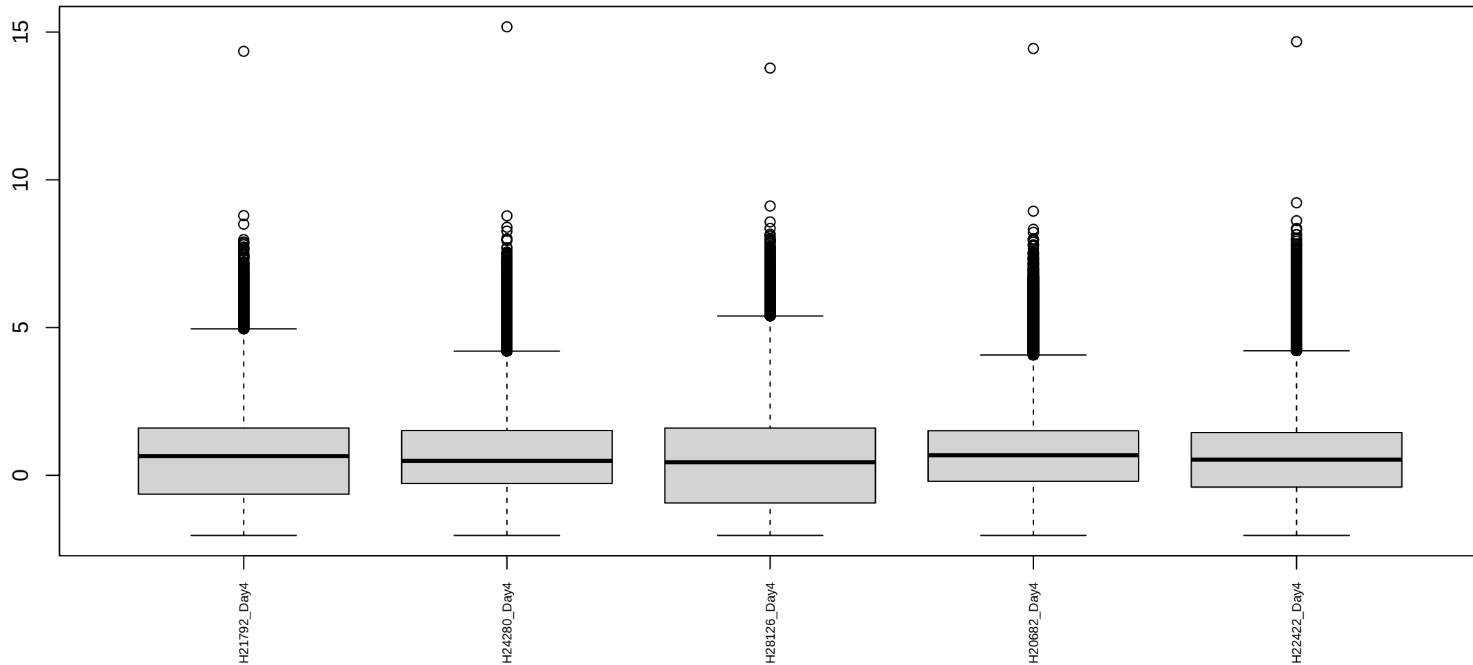
Boxplots of log cpm per sample Human Day 4 Reproducible2
