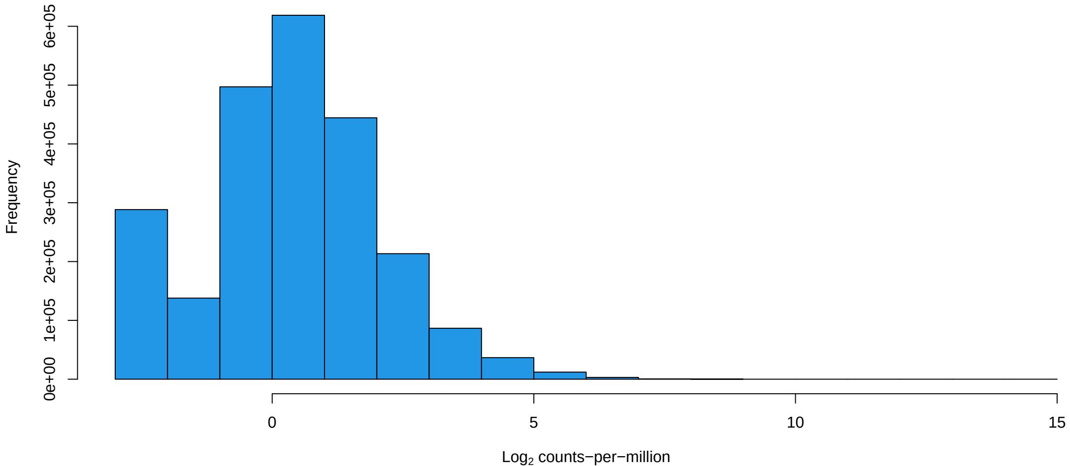
Histogram of all counts – Human Day 5 Reproducible2
