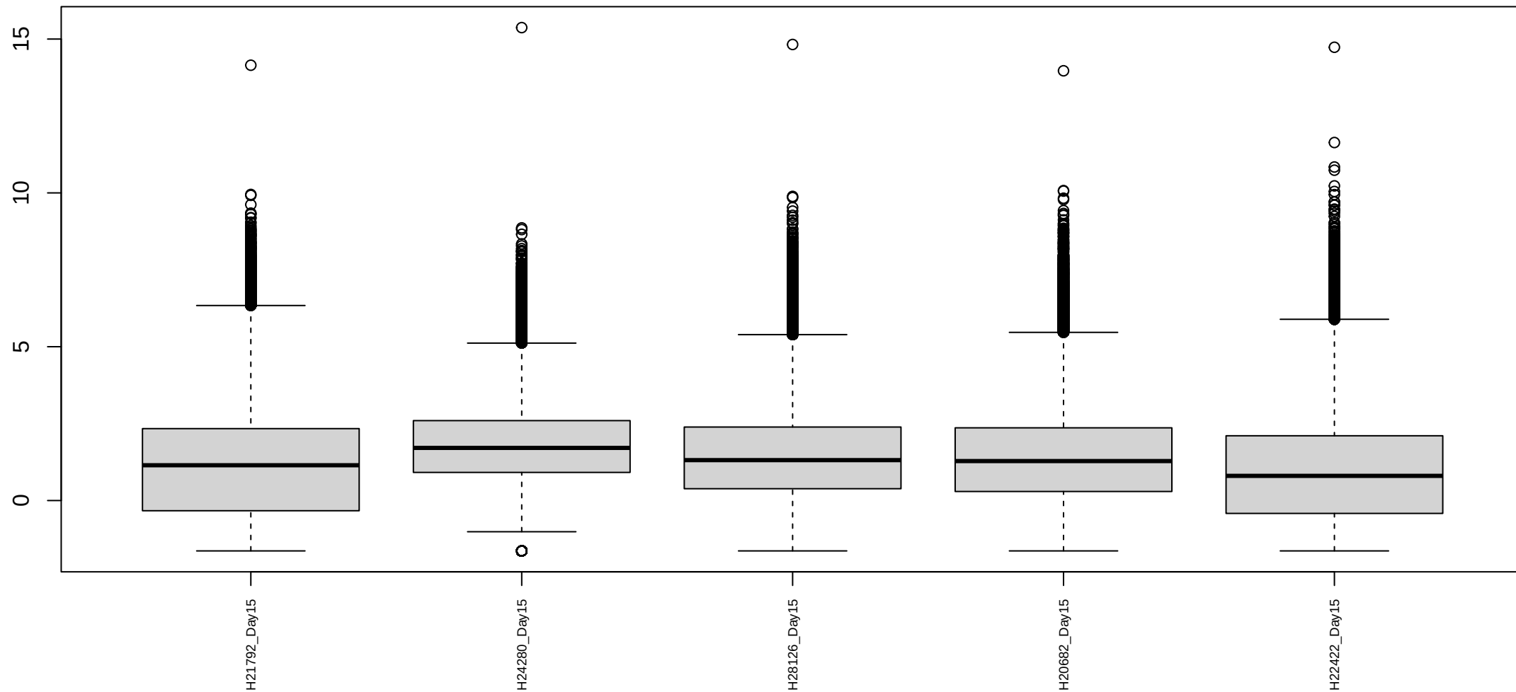
Boxplots of log cpm per sample Human Day 15 Reproducible3
