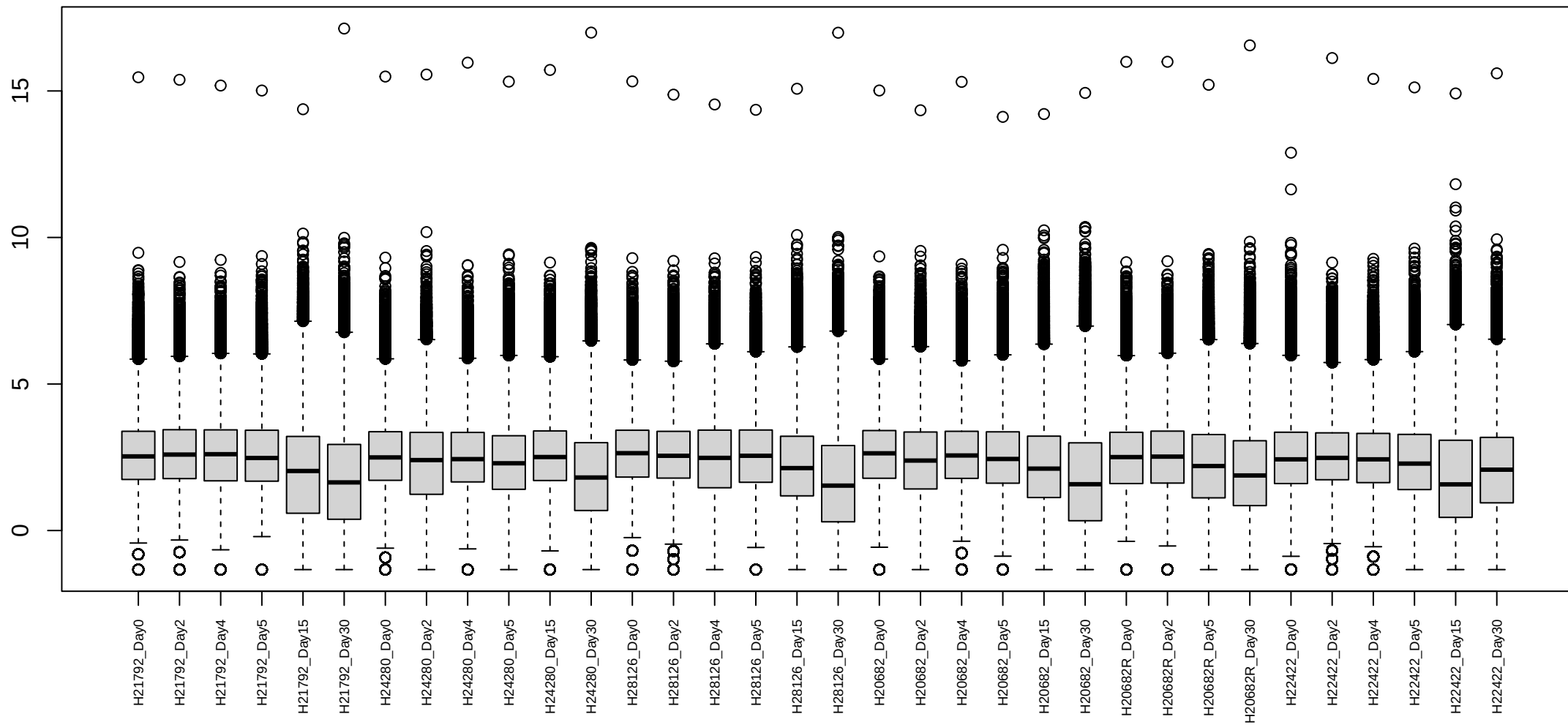
Boxplots of log cpm per sample Human Reproducible4
