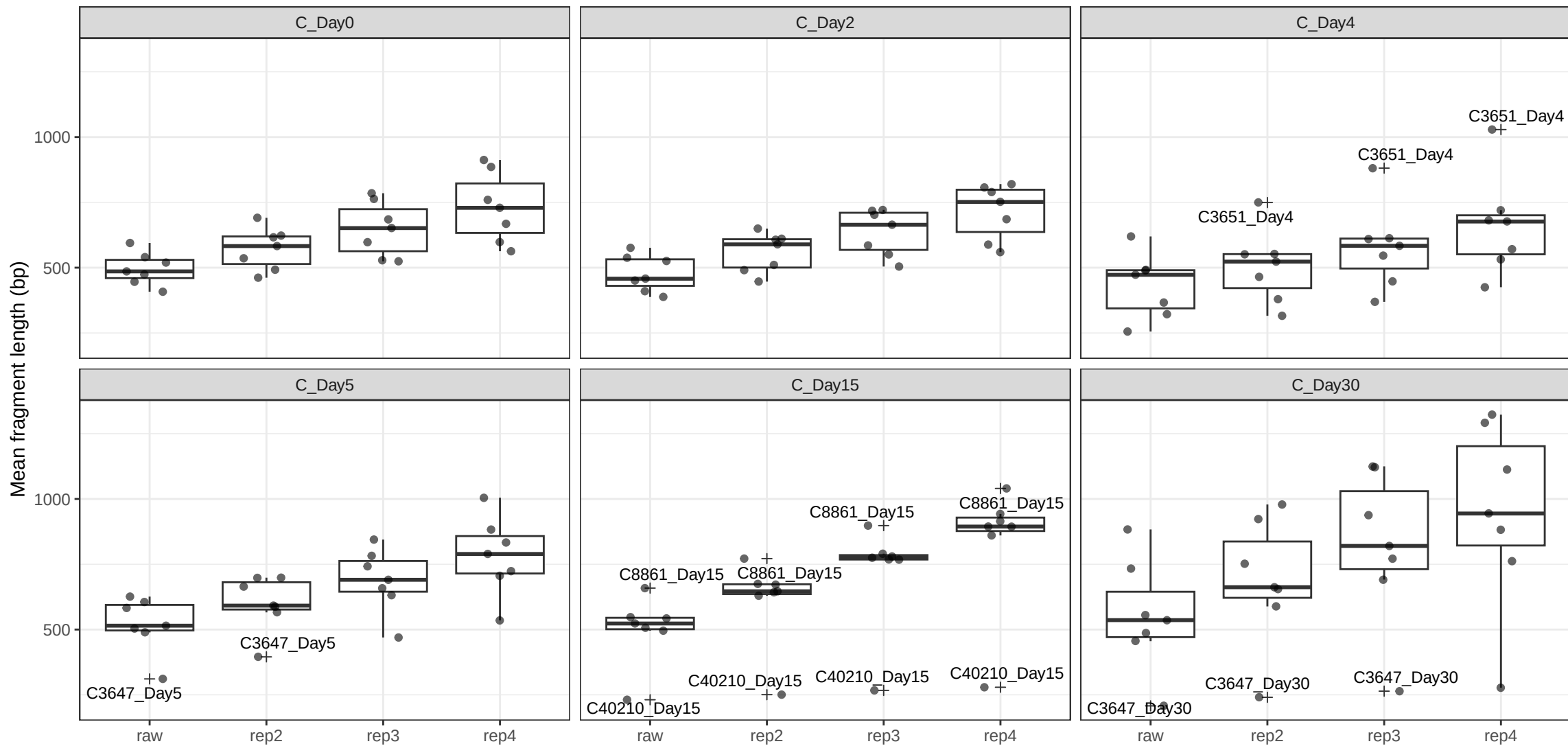
C samples: fragment length
