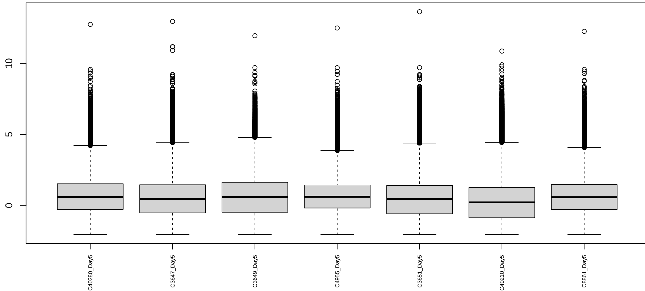
Boxplots of log cpm per sample Chimp Day 5 Reproducible2
