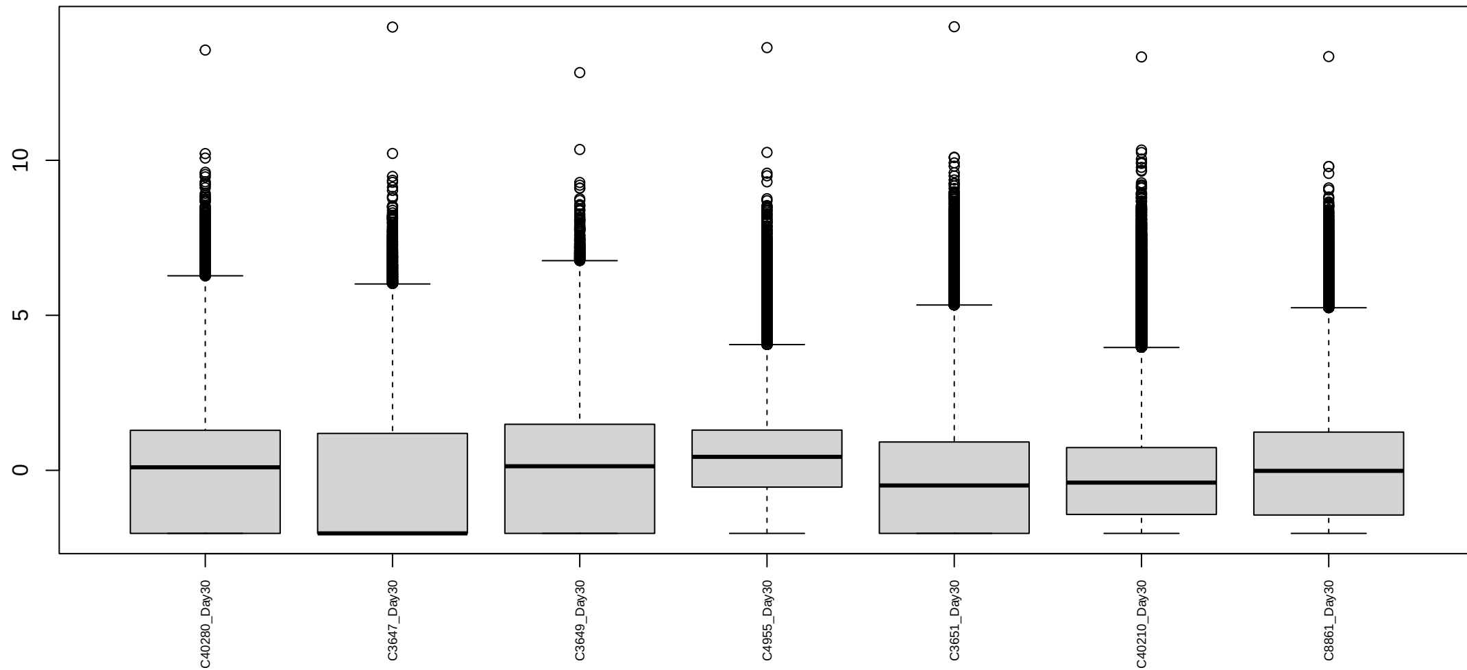
Boxplots of log cpm per sample Chimp Day 30 Reproducible2
