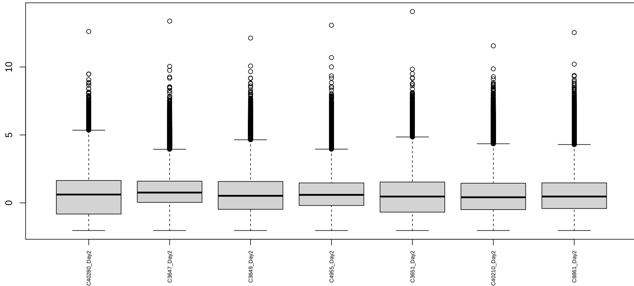
Boxplots of log cpm per sample Chimp Day 2 Reproducible2
