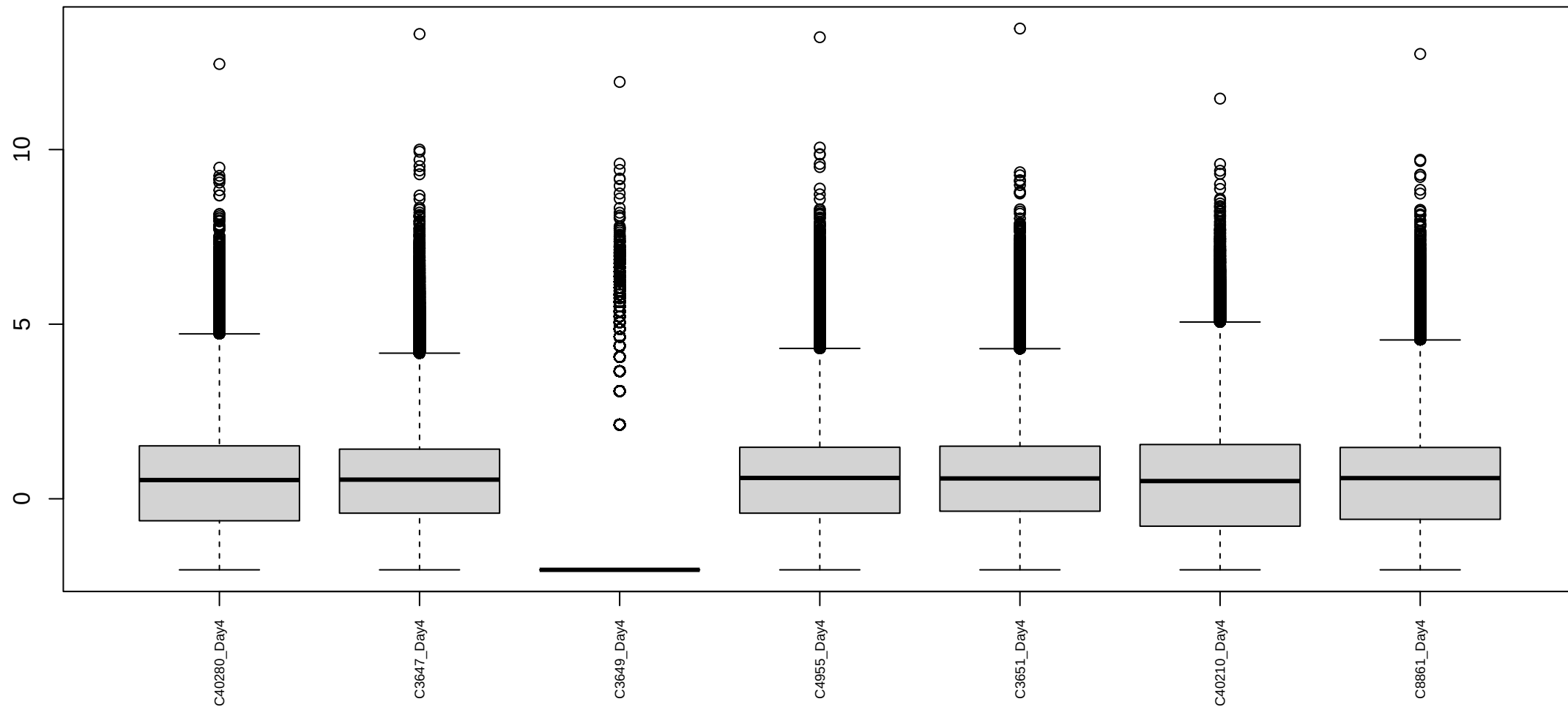
Boxplots of log cpm per sample Chimp Day 4 Reproducible2
