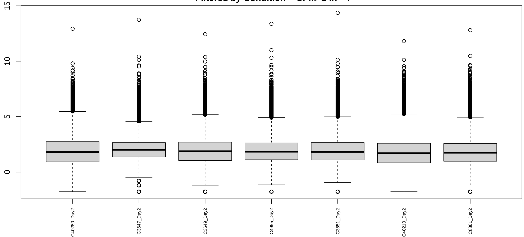
Boxplots of log cpm per sample Chimp Day 2 Reproducible2 Filtered by Condition – CPM>2 in >4
