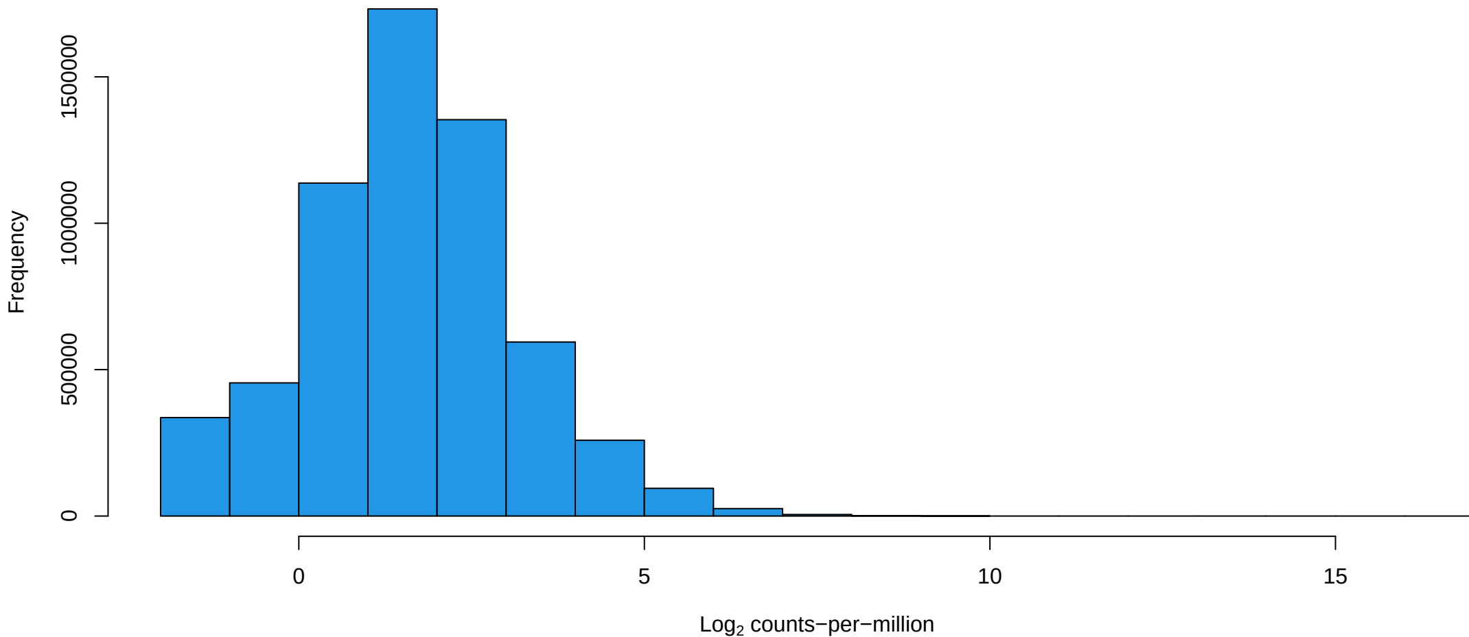
Histogram of all counts – Human Reproducible2 Filtered by Condition – CPM>2 in >4
