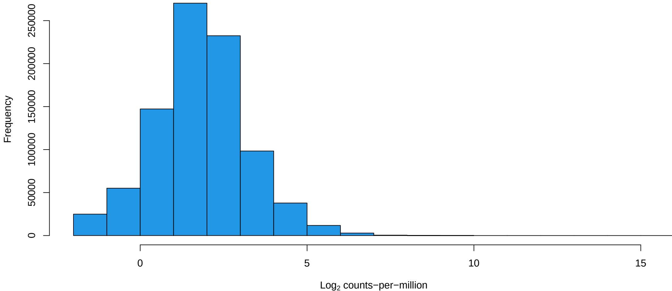
Histogram of all counts – Human Day 4 Reproducible2 Filtered by Condition – CPM>2 in >4
