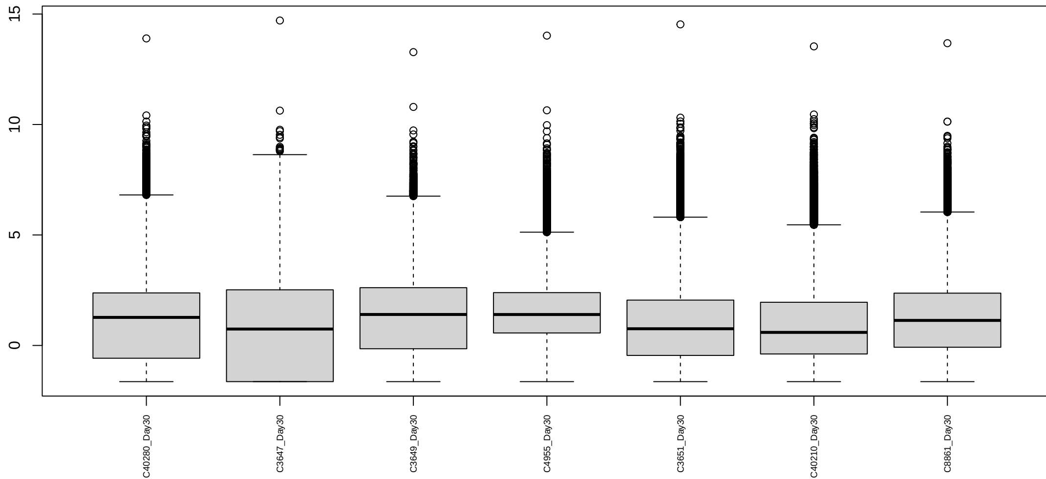
Boxplots of log cpm per sample Chimp Day 30 Reproducible3
